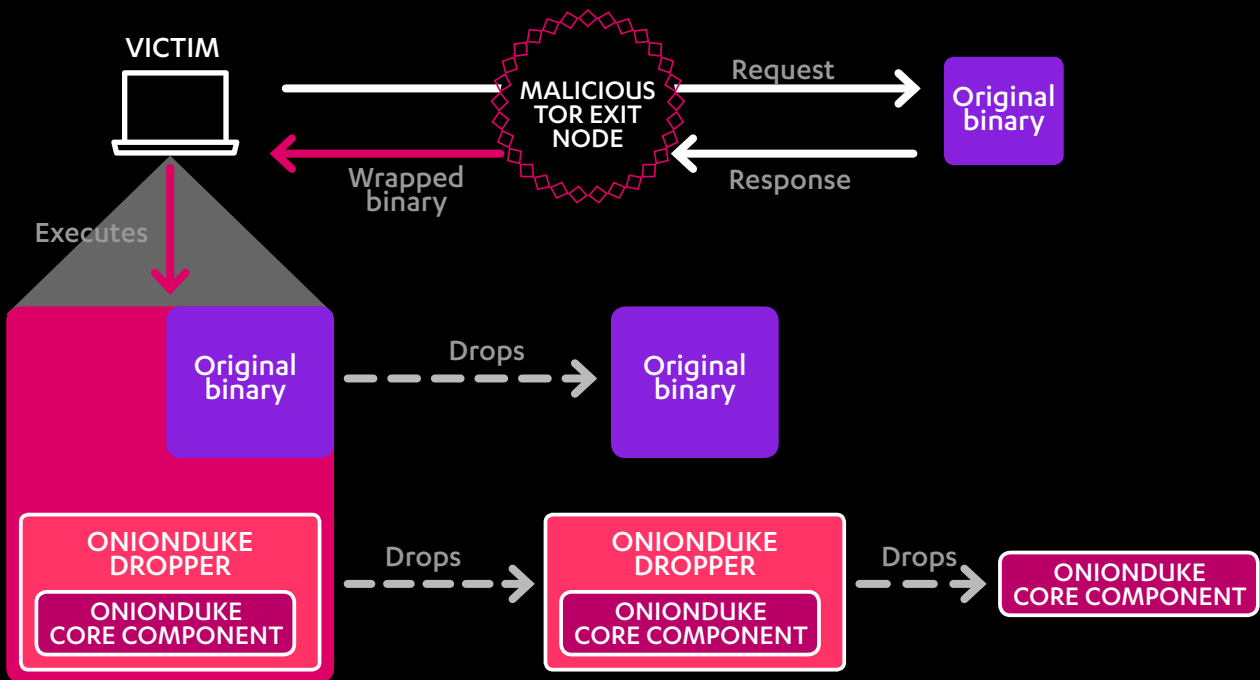
IMAGE 7: FLOWCHART OF HOW ONIONDUKE USES MALICIOUS TOR NODE TO INFECT VICTIMS
